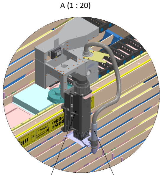
THC Ünitesi THC Unit Plazma Torchu Plasma Torch
